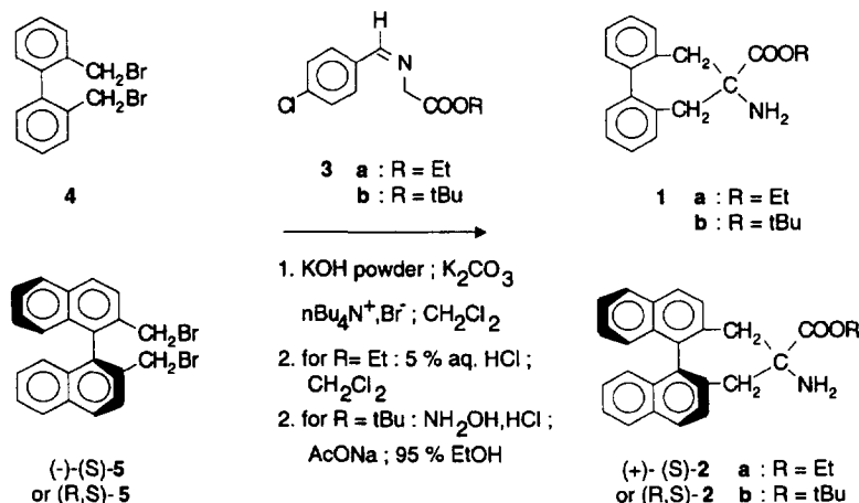
Figure 2. Synthesis of the aminoesters H-Bip-OEt ( 1a ), H-Bip-OtBu ( 1b ), H-Bin-OEt ( 2a ) and H-Bin-OtBu ( 2b ) under phase transfer conditions.
