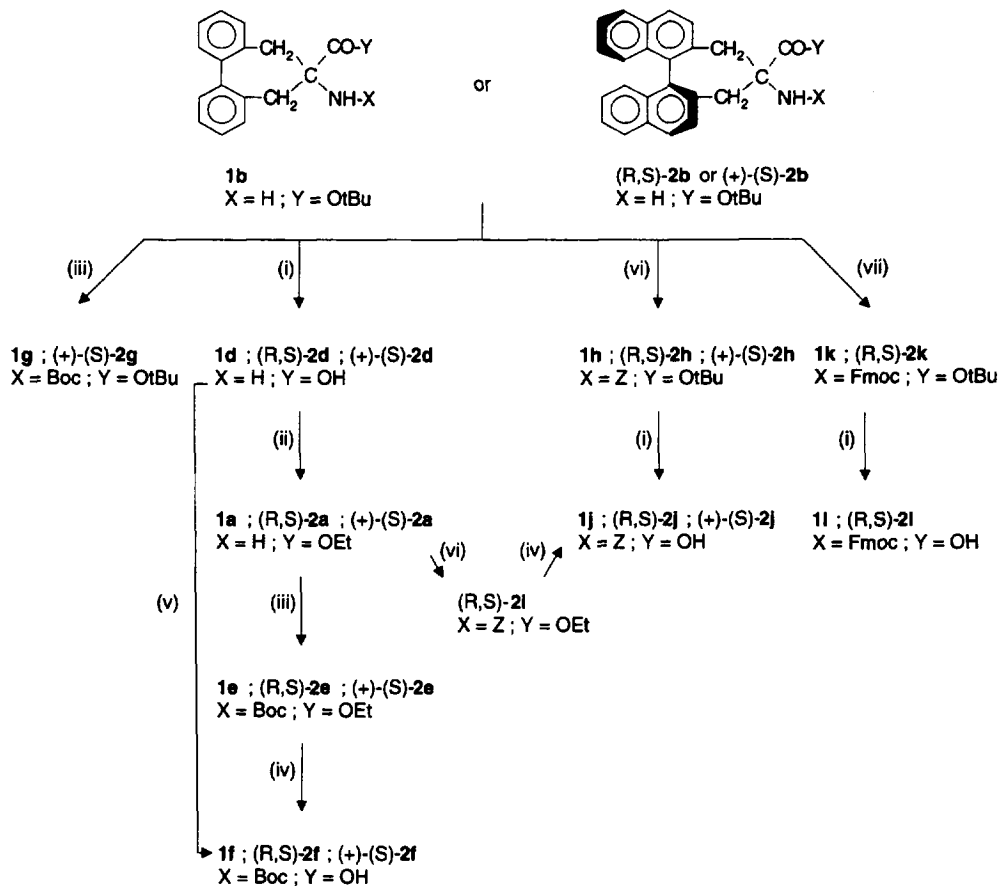
Figure 3. Synthesis of the C- and/or N-protected derivatives of Bip and Bin. (i) TFA/CH 2 Cl 2 1:1; rt; 2 h (ii) abs. EtOH; H 2 SO 4 ; reflux; 48 h (iii) Boc 2 O; CH 3 CN; rt; 24 h (iv) aq. N NaOH/MeOH; 75°C; 2–3 h (v) Boc 2 O; N NaOH; dioxane; rt; 12 days or Boc 2 O; Et 3 N; CH 3 CN; rt; 48 h (vi) Z-OSu; CH 3 CN; rt; 24 h (vii) Fmoc-OSu; CH 3 CN; rt; 24 h.
