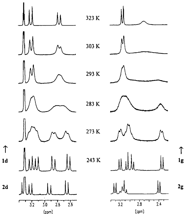
Figure 4. Temperature-dependent 300 MHz ^1\text{H} NMR pattern of (\text{ArCH}_2 \beta)(\text{Ar}'\text{H}_2 \beta) for the compounds H-Bip-OH ( 1d ) in \text{CD}_3\text{OD} and Boc-Bip-OtBu ( 1g ) in \text{CDCl}_3 (c 20 g/l), compared to their conformationally stable analogs 2d and 2g at room temperature (294 K). 1d : T_{\text{C}1}=278 K ( \Delta\nu_1=28.3 Hz); T_{\text{C}2}=288 K ( \Delta\nu_2=71.3 Hz). 1g : T_{\text{C}1}=283 K ( \Delta\nu_1=44.3 Hz); T_{\text{C}2}=303 K ( \Delta\nu_2=184.8 Hz).
